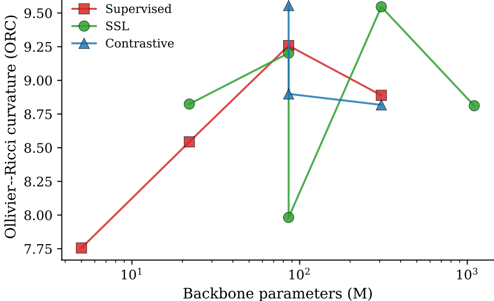
MNIST -- ORC vs. backbone scale
