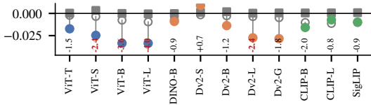
(a) ImageNet, WordNet K = 30 ( n = 1000 )
