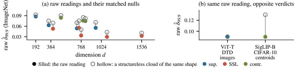
Figure 2: The raw reading cannot be read on its own. (a) Each ImageNet backbone’s raw reading (filled) and what a structureless cloud of the same dimension and spectrum reads (hollow); the nulls drift down with the dimension, and the segment between the two is the excess. (b) Two cells with the same raw reading and opposite verdicts: on ViT-T image features the null sits at the reading, on SigLIP-B centroids far above it.
