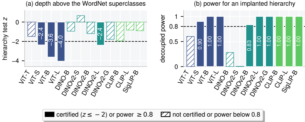
Figure 4: What the hierarchy test certifies, and where it can see a hierarchy. (a) Depth z per backbone, filled when certified; line at z = -2 . (b) Decoupled power for an implanted three-level hierarchy, filled at 0.8 or more; line at 0.8.
