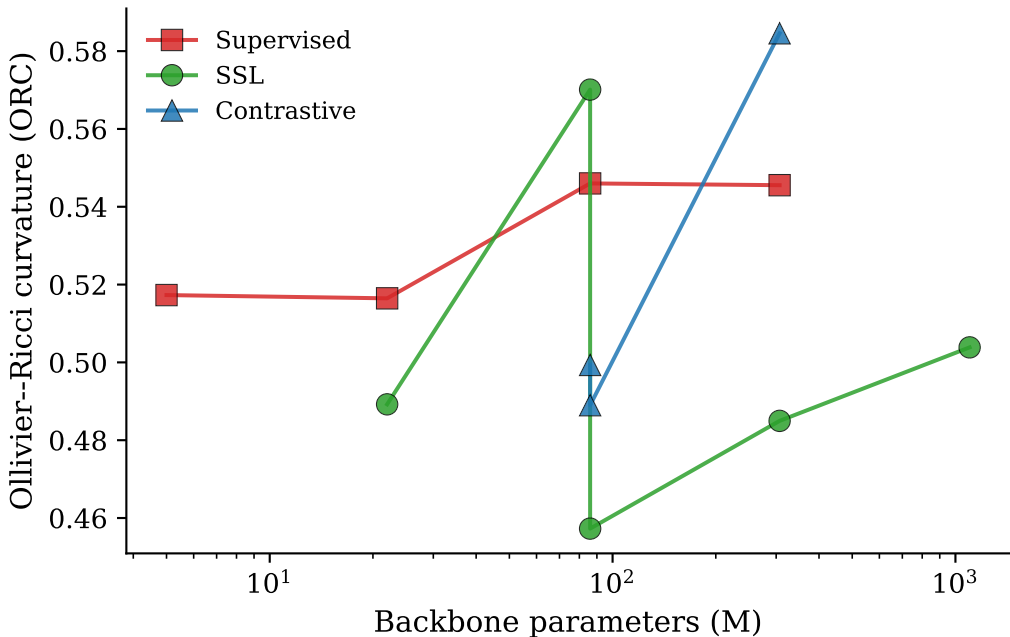
FashionMNIST -- ORC vs. backbone scale
