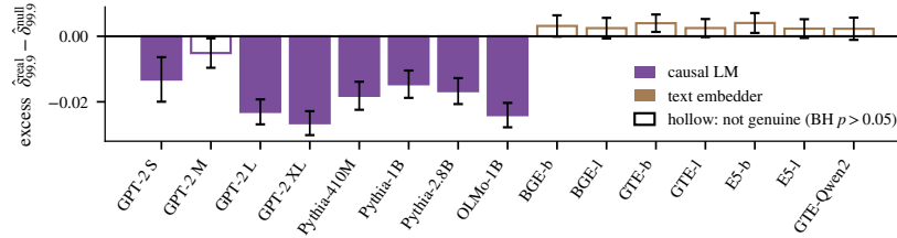
Figure 10: In text, clustered structure depends on recipe and scale: robust at the larger GPT-2 sizes, fragile at the smaller. Plotted: the text census of record (padding-free extraction, Haar null, 99.9th-percentile statistic, 200 replicates), with error bars combining null and estimator s.d., hollow bars for cells that are not genuine, and OLMo-7B omitted as not re-extracted.
