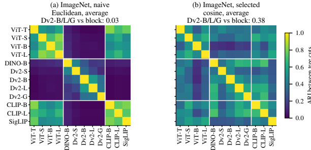
Figure 5: The categorical island is a chaining artifact; about a third of the within-block agreement is missing under most configurations. Plotted: pairwise ARI between the dendrogram cuts of the 12 vision models on ImageNet under the naive configuration (a) and the selected one (b), with the mean DINOv2-vs-block ARI above each panel.
