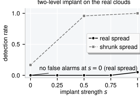
Figure 7: A two-level implant on the real ImageNet clouds is missed at the real within-cluster spread and detected once the spread is shrunk. Detection rate at z \leq -2 against implant strength s with the real within-cluster spread (solid) and shrunk (dashed): at full strength 0.05 against 1.00, and 0.00 at s = 0 with the real spread.
