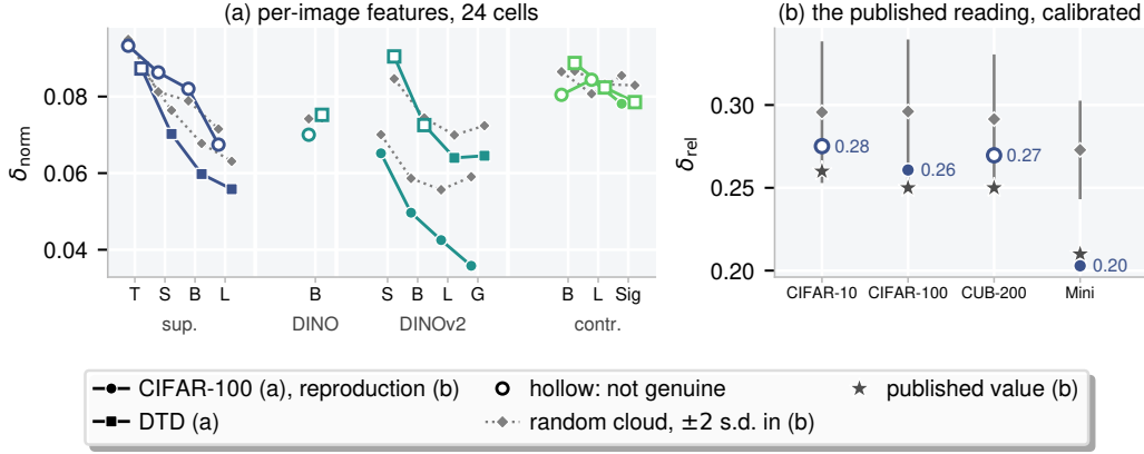
Figure 3: The premise where it is read. (a) Per-image features: raw reading and a random cloud of the same shape; filled dots are genuine. (b) The published values, their reproduction and the random cloud: two of four are indistinguishable from it, on their statistic, the supremum; filled and hollow dots follow the reading, which gives the same verdict.
