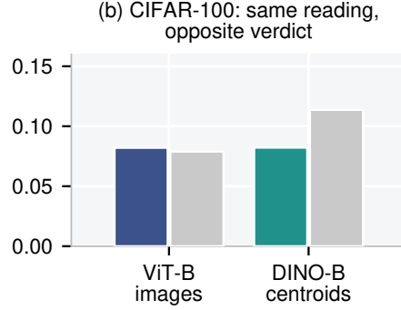
Figure 6: The same reading, opposite verdicts. The raw reading of ViT-B on CIFAR-100 images and of DINO-B on CIFAR-100 centroids, each beside the mean of its matched null: the same reading, and only one of them is genuine.
