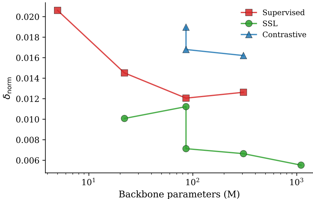
ImageNet -- delta vs. backbone scale
