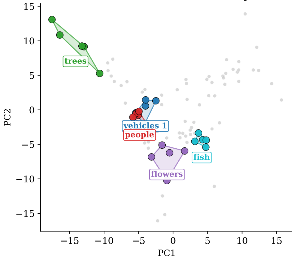
(a) Euclidean: PCA in raw feature space
