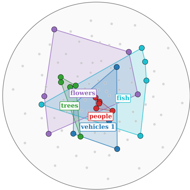
(b) Poincaré disk: hyperbolic-MDS on d_{\mathbb{B}}(\phi(\cdot))
