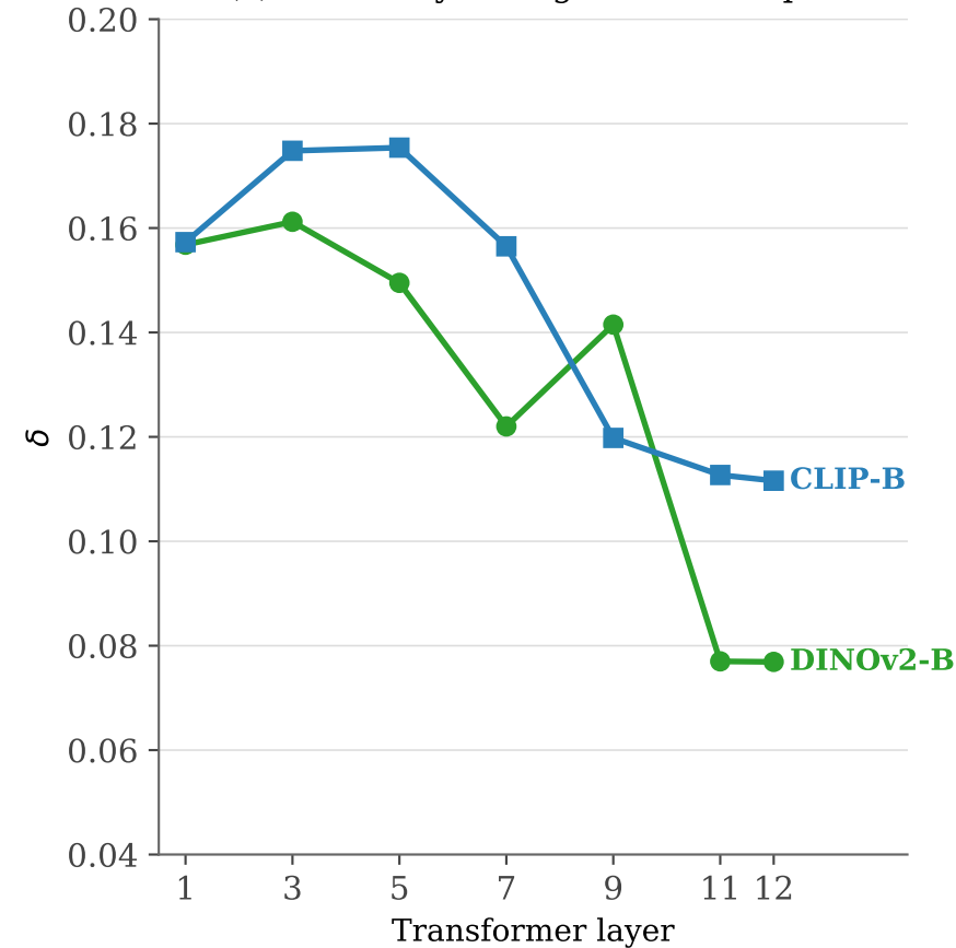
(c) Hierarchy emerges across depth
