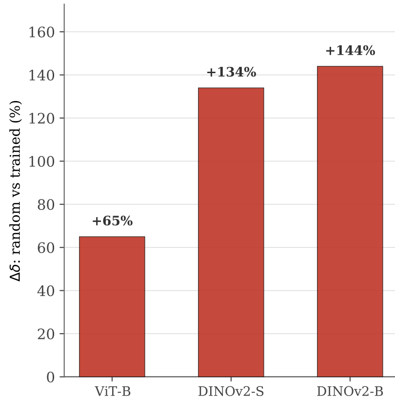
(a) Random weights inflate \delta
