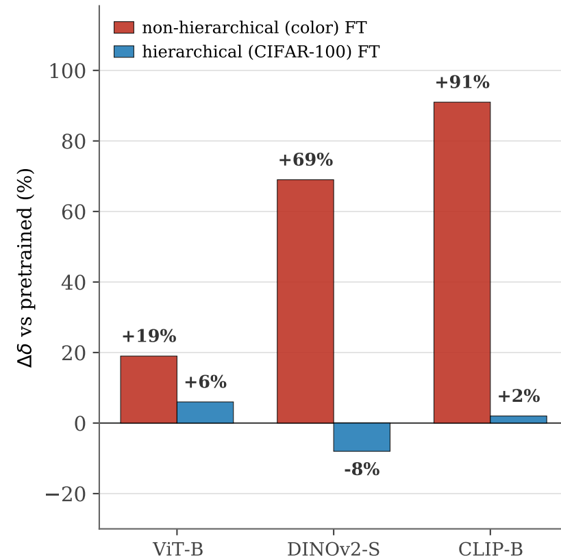
(b) Non-hierarchical fine-tuning inflates \delta
