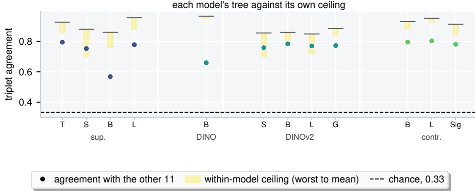
Figure 10: Every tree stays under its own ceiling and well above chance. Per backbone: triplet agreement with the other 11 (dot) against the band of its own bootstrap copies, worst to mean.
