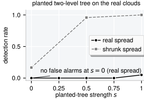
Figure 8: A planted two-level tree on the real ImageNet clouds is missed at the real within-cluster spread and detected once the spread is shrunk. Detection rate at z \leq -2 against planted-tree strength s with the real within-cluster spread (solid) and shrunk (dashed): at full strength 0.05 against 1.00, and 0.00 at s = 0 with the real spread.
