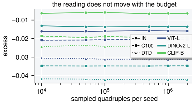
Figure 7: The reading does not move with the quadruple budget. Excess against the number of sampled quadruples per seed, one line per cell: 3 backbones on ImageNet, CIFAR-100 and DTD.
