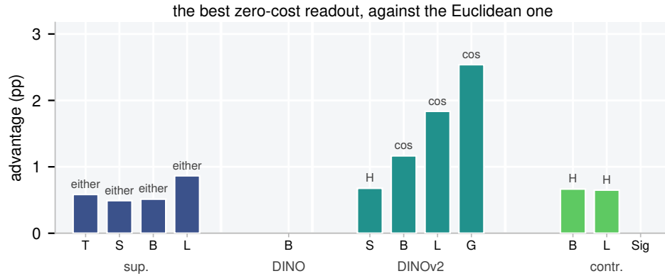
Figure 11: The zero-cost advantage is small and largest for the self-supervised models. Best few-shot advantage over the Euclidean readout per backbone, averaged over the 4 hierarchical datasets, with the metric that collects it.
