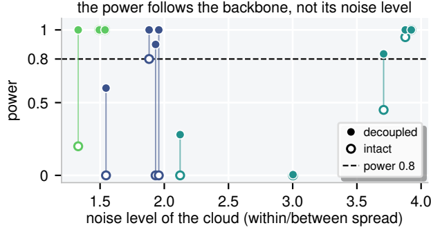
Figure 9: The power follows the backbone, not the noise level of its cloud. Power against the within/between spread per backbone, intact (hollow) and decoupled (filled); dashed: power 0.8.
