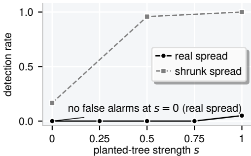
planted two-level tree on the real clouds
