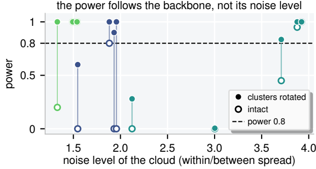
Figure 8: The power follows the backbone, not the noise level of its cloud. Power against the within/between spread per backbone, intact (hollow) and with clusters rotated (filled); dashed: power 0.8.
