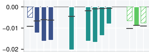
(b) excess over the random cloud
