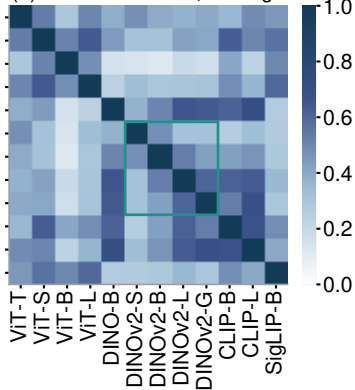
(b) selected: cosine, average ARI
