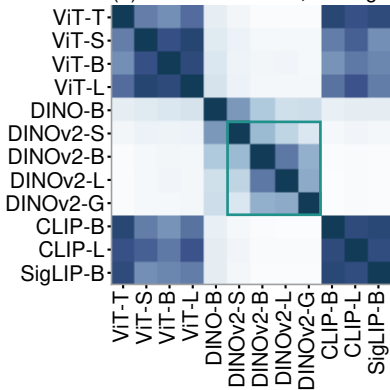
(a) naive: Euclidean, average
