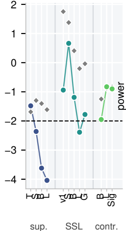
(c) hierarchy test, intact and randomized
