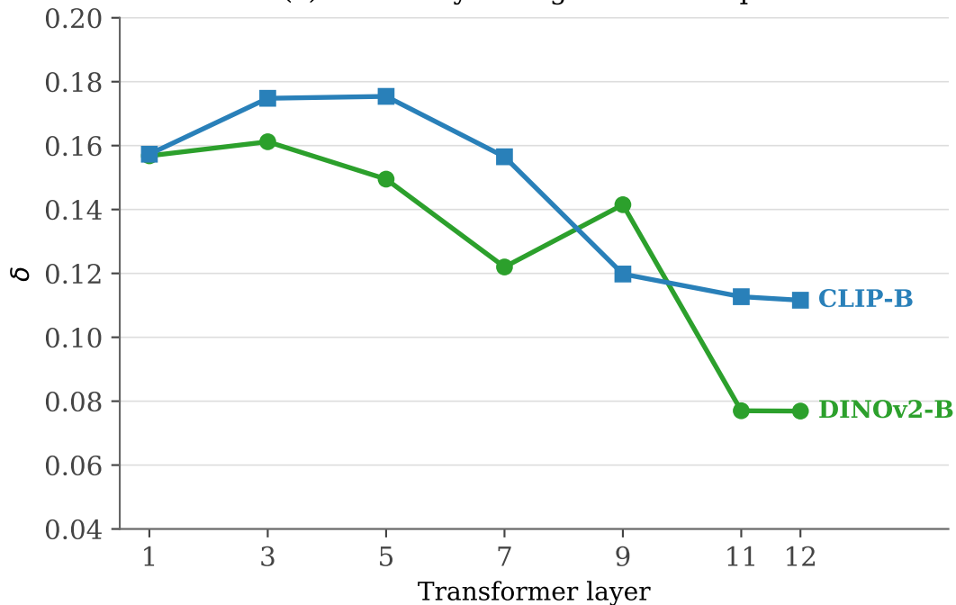
(c) Hierarchy emerges across depth
