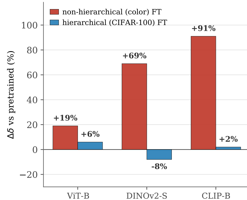
(b) Non-hierarchical fine-tuning inflates \delta
