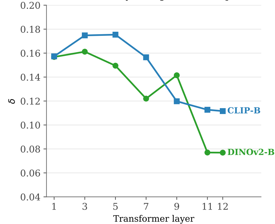
(c) Hierarchy emerges across depth
