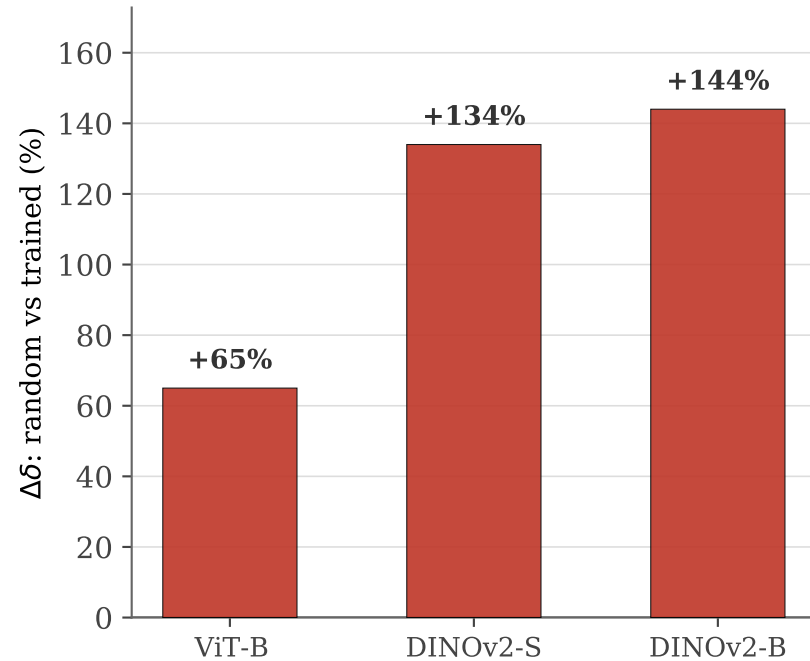
(a) Random weights inflate \delta
