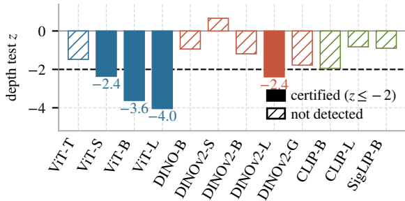
(a) depth above the WordNet superclasses, ImageNet
