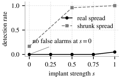
(b) false alarms and power on real clouds
