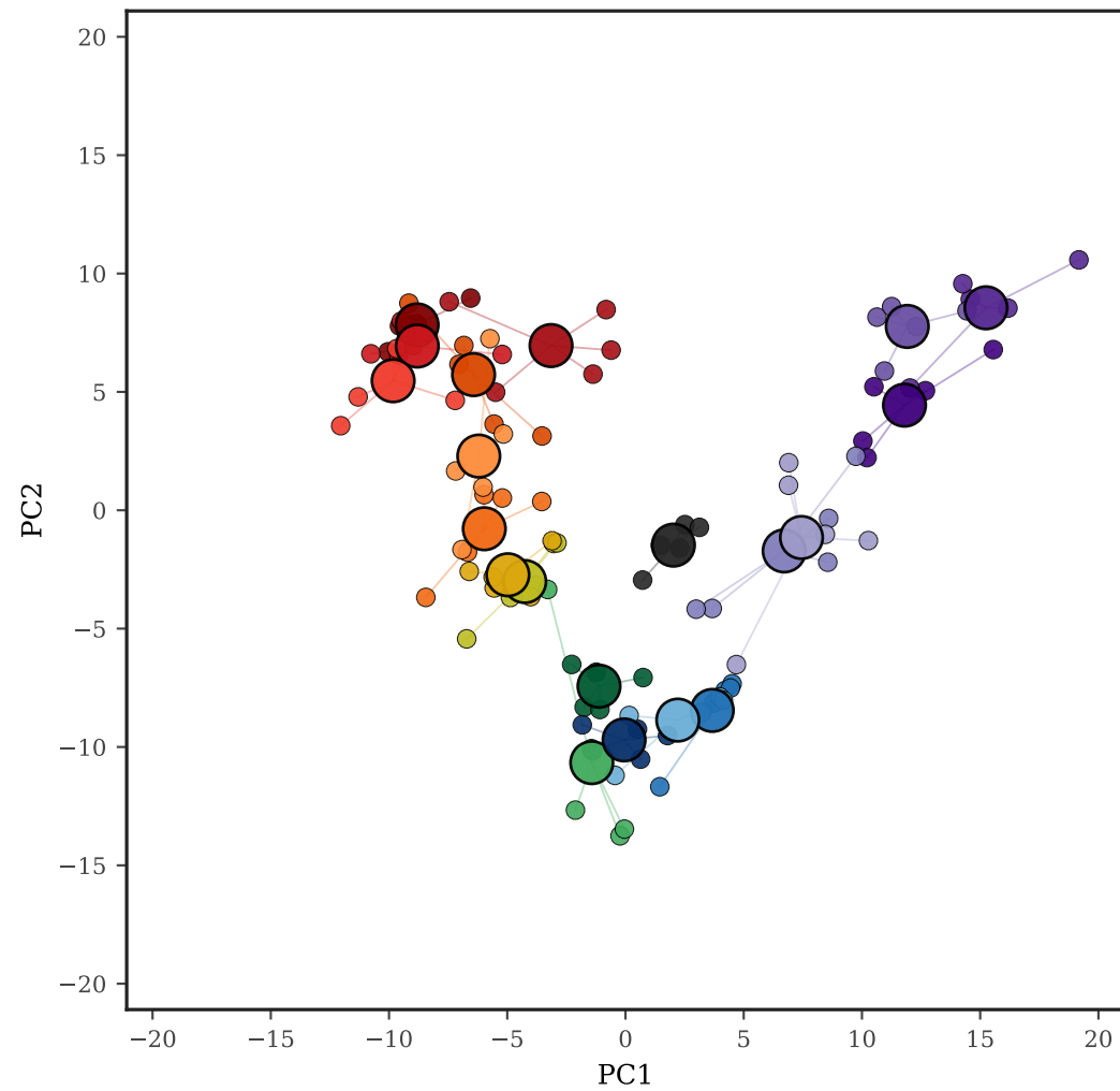
(a) DINOv2-S - Euclidean \delta = 0.107
