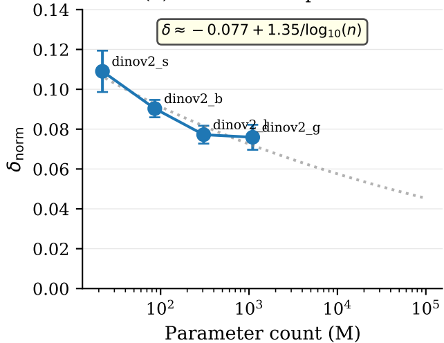
(b) DINOv2 extrapolation
