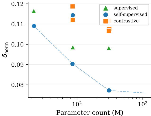
(a) Divergence across paradigms
