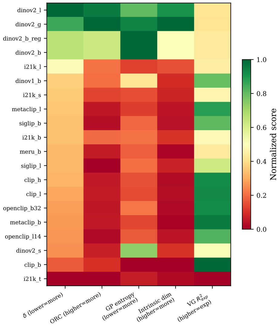
Hyperbolicity scorecard (green = more hyperbolic)
