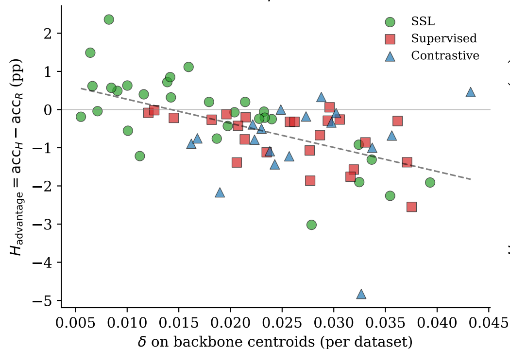
NC: Nearest-Centroid
