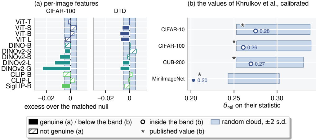
Figure 3: The premise where it is read. (a) Excess of the reading on per-image features; filled: genuine, 10 of 24 cells. (b) The values reported by Khrulkov et al. (2020), our reproduction with their estimator, and the random cloud of the same shape, all on their statistic: a dot inside the band is what chance gives. On their statistic CIFAR-10 and CUB-200 fall inside the band, MiniImageNet below it, and CIFAR-100 at its edge, its verdict changing from trial to trial (median rank 196/200); on our reading only MiniImageNet is genuine after correction, and CIFAR-100 falls below at p = 0.030 before it (Section 5.1).
