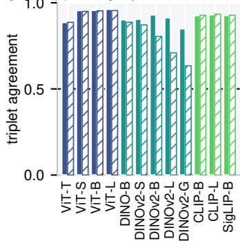
(c) sibling triplets, CIFAR-100
