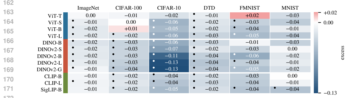
Figure 3: Clustered structure is the rule at the class level. Excess of the reading of record over its matched null for the 12 backbones on 6 datasets; dots mark genuine cells. Almost every cell is below its null, most are genuine, the flat datasets sit near zero, and the excess deepens down the DINOv2 rows on CIFAR-10.
