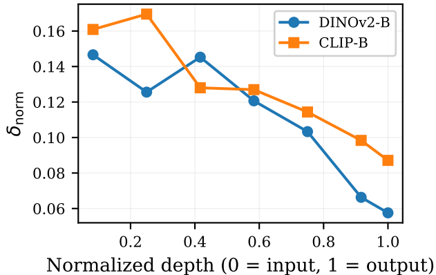
\delta across transformer layers
