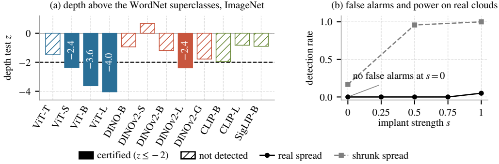
Figure 4: The alignment of each cluster with its hub is certified in 4 of 12 ImageNet backbones; no hierarchy above the superclasses is found. (a) Depth z per backbone under the matched star, filled and numbered when certified, hatched otherwise; certification line at z = -2 . (b) Detection rate against implant strength on the real clouds with the real within-cluster spread (solid) and shrunk into the range where false alarms are controlled (dashed).
