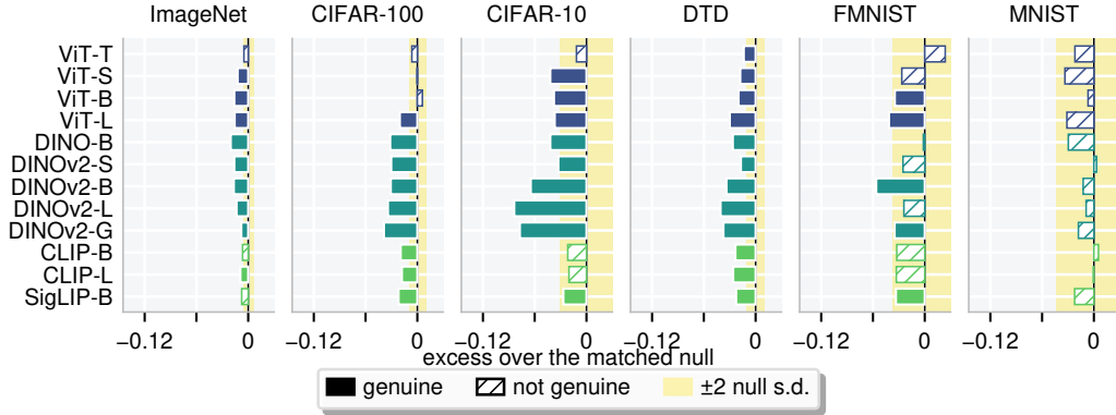
Figure 4: Most cells show structure beyond the second moments. Excess of the reading over its matched null per dataset and backbone, filled when genuine; band: two null standard deviations.
