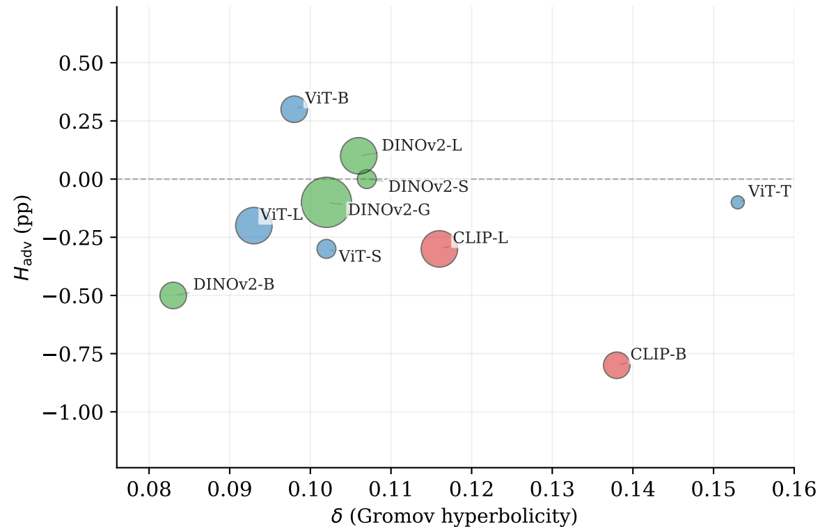
(a) NC: nearest-centroid
