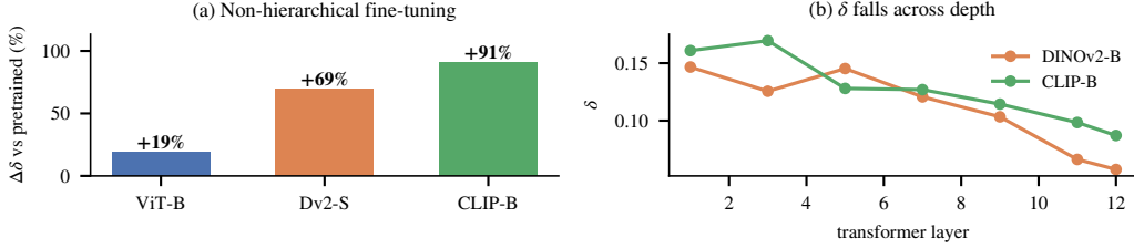
Figure 5: The form is learned: training interventions move it. Raw \delta , within architecture. (a) Non-hierarchical fine-tuning raises \delta 19–91%. (b) \delta falls across transformer depth (layers \geq 1 ).
