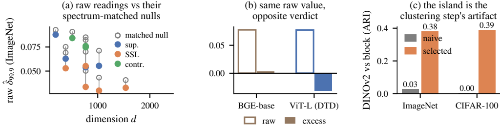
Figure 2: Why calibration: raw \delta cannot be read on its own, and naive tree comparison manufactures islands. (a) Raw \delta_{99.9} of the 12 backbones on ImageNet against their spectrum-matched null means (hollow): the raw value tracks dimension and spectrum, the gap is the reading. (b) A text embedder (BGE-base) and a vision cell (ViT-L on DTD) share the same raw value with opposite null verdicts. (c) DINOv2-vs-block tree agreement before and after the configuration control of §5.
