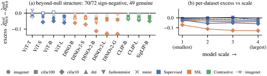
Figure 3: Beyond-null (clustered) structure in most vision cells and every family. (a) Excess of the 99.9th-percentile statistic over its Haar spectrum-matched null per cell (12 models \times 6 datasets; hollow markers: not genuine, BH p > 0.05 ). (b) Per-dataset excess vs scale: only DINOv2 on CIFAR-10 (and weakly on CIFAR-100) deepens monotonically; cross-dataset magnitudes are not comparable.
