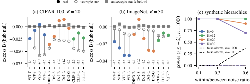
Figure 7: The matched-star depth test, reported as not validated. (a,b) Excess B under the hub-randomizing null for the real centroids (filled, family colors) and for matched stars (hollow circle: isotropic; square: anisotropic), CIFAR-100 ( K=20 ) and ImageNet ( K=30 ); the number under each backbone is the z of real minus anisotropic star (negative = more hierarchical above the frame). (c) Power ( z \leq -2 ) on synthetic hierarchies with n=1000 and the frame at the leaf clusters (solid, one line per K ) or at the top level (dotted, zero by construction); dashed: false alarms ( z \leq -2 ) on pure stars at n=1000 (gray) and n=100 (black).
