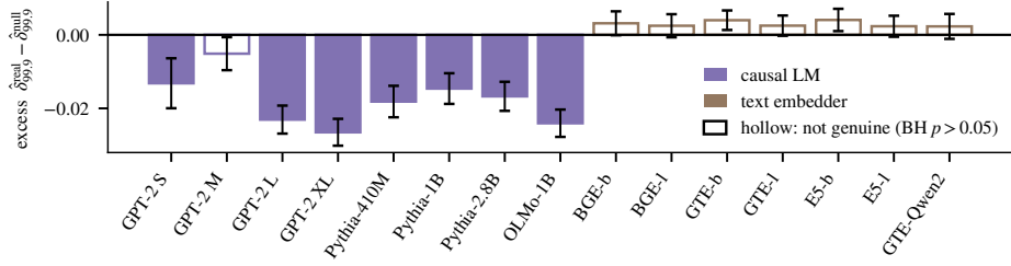
Figure 4: In text, beyond-null structure depends on recipe and scale: robust at the larger GPT-2 sizes, fragile at the smaller. Text census of record (padding-free extraction, Haar null, 99.9th-percentile statistic, 200 replicates; error bars combine null and estimator s.d.; hollow bars are not genuine, BH p > 0.05 ; OLMo-7B, not re-extracted, omitted). Pythia and OLMo-1B are genuine throughout; classic sentence embedders are not on this probe despite raw values equal to genuinely structured vision models.
