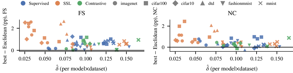
Figure 9: More tree-like cells carry larger zero-cost metric gains. Best zero-cost metric minus Euclidean per cell vs \delta_{\text{norm}} (FS left, NC right). Within-dataset correlations -0.60 to -0.83 (FS) and -0.61 to -0.86 (NC); pooled correlations are family-driven and not used as evidence (Appendix A.12).
