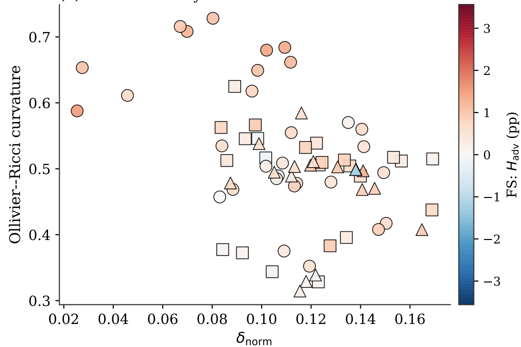
(b) Few-shot 5-way 5-shot
