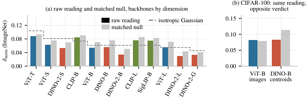
Figure 2: The raw reading cannot be read on its own. (a) Raw reading and matched null per ImageNet backbone, ordered by dimension; the gap is the excess. (b) Same dataset, same reading, opposite verdict: ViT-B on CIFAR-100 images and DINO-B on CIFAR-100 centroids.
