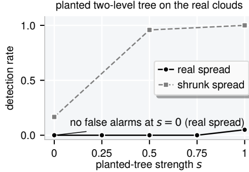
Figure 9: A planted two-level tree on the real ImageNet clouds is missed at the real within-cluster spread and detected once the spread is shrunk. Detection rate at z \leq -2 against planted-tree strength s with the real within-cluster spread (solid) and shrunk (dashed): at full strength 0.05 against 1.00, and 0.00 at s = 0 with the real spread.
