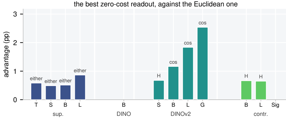
Figure 12: The zero-cost advantage is small and largest for the self-supervised models. Best few-shot advantage over the Euclidean readout per backbone, averaged over the 4 hierarchical datasets, with the metric that collects it.
