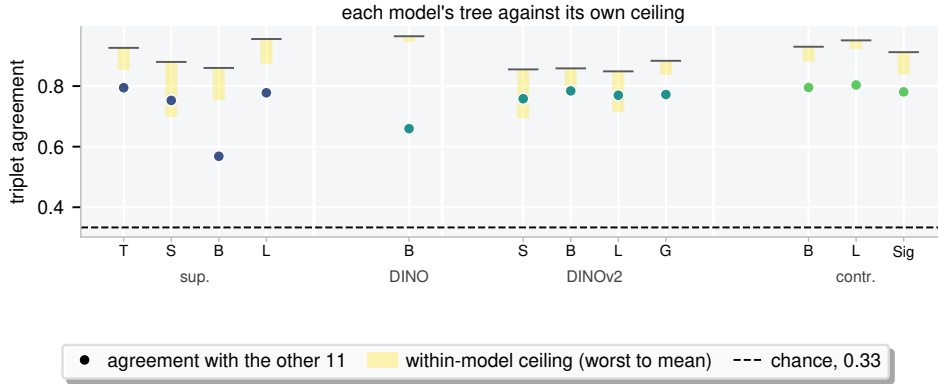
Figure 11: Every tree stays under its own ceiling and well above chance. Per backbone: triplet agreement with the other 11 (dot) against the band of its own bootstrap copies, worst to mean.
