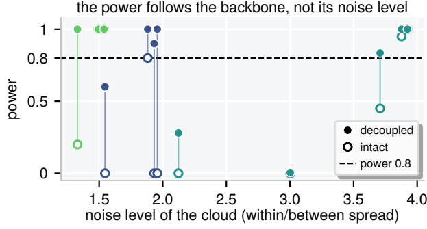
Figure 10: The power follows the backbone, not the noise level of its cloud. Power against the within/between spread per backbone, intact (hollow) and decoupled (filled); dashed: power 0.8.
