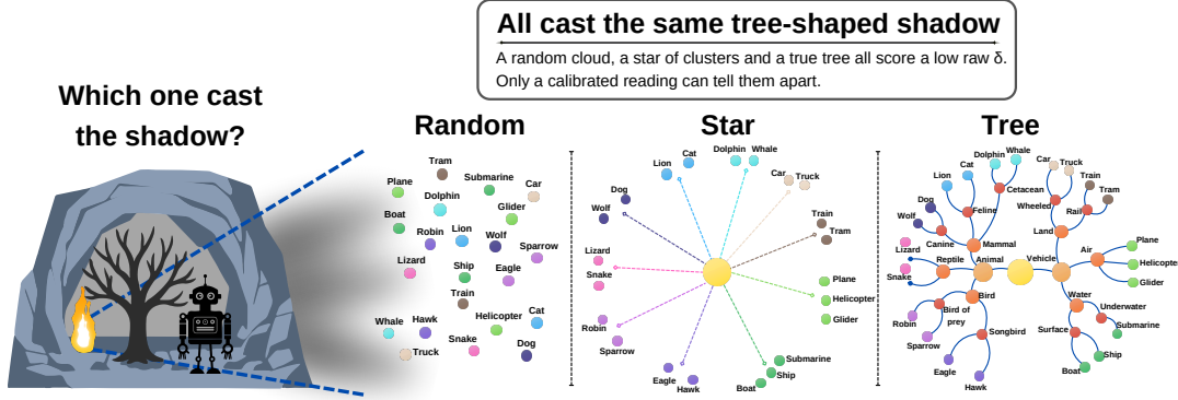
Figure 1: Plato’s cave: a random cloud, a star and a tree cast the same shadow. An observer who sees only shadows cannot tell which object cast them, and a raw \delta is such a shadow: points with no structure, clusters around a hub, and a nested hierarchy all read as low \delta . The instrument reads the objects instead of the shadow: the excess separates the random cloud from the other two, and the hierarchy test separates the star from the tree.
