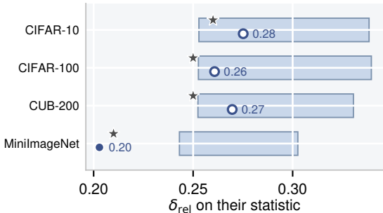
(b) the values of Khrulkov et al., calibrated
