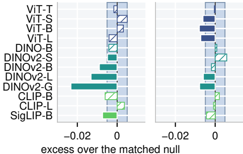
(a) per-image features
