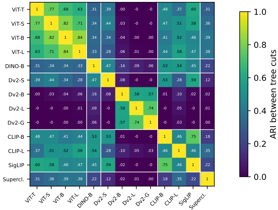
(b) CIFAR-100, ARI @ 20 clusters
