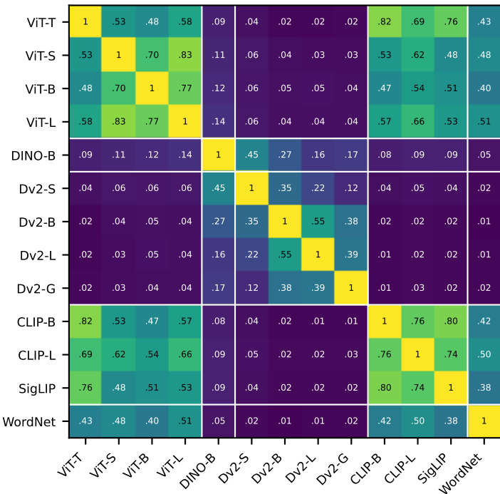
(a) ImageNet, ARI @ 30 clusters
