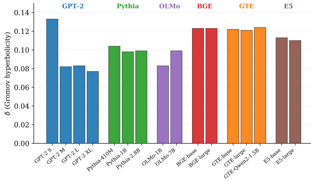
(c) Text: \delta by family
