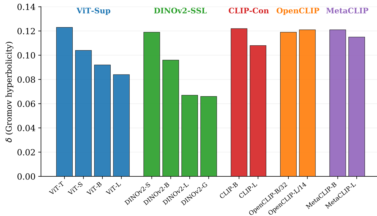
(a) Vision: \delta by family
