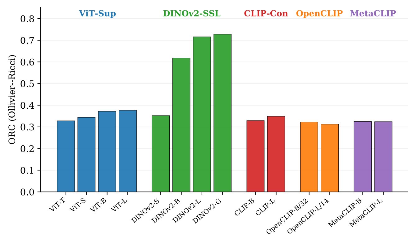
(b) Vision: ORC by family
