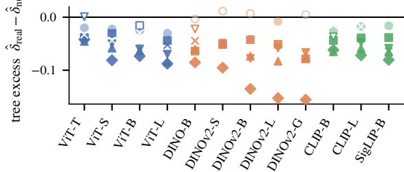
(a) 68/72 cells below their matched null
