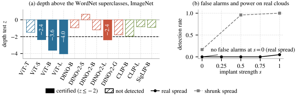
Figure 4: The depth test certifies in 4 of 12 ImageNet backbones that clusters are oriented toward their hubs, not that the hubs form a hierarchy; no hub hierarchy is found in the five backbones where the control detects an implanted one, and the test is blind in the other seven. (a) Depth z per backbone, filled when certified; line at z = -2 . (b) Detection rate against implant strength with the real within-cluster spread (solid) and shrunk (dashed).
