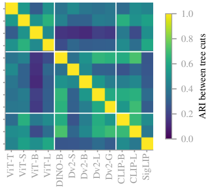
(b) ImageNet, selected cosine, average Dv2-B/L/G vs block: 0.38
