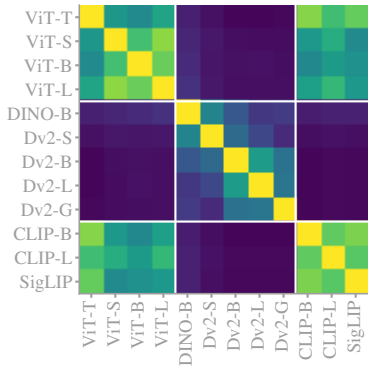
(a) ImageNet, naive Euclidean, average Dv2-B/L/G vs block: 0.03
