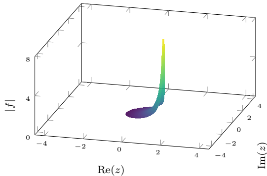
(b) Taylor: |z| < 1
