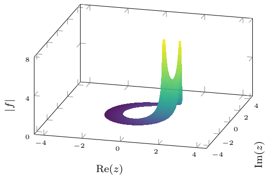
(c) Laurent: 1 < |z| < 2
