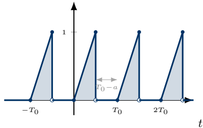
(c) y(t) = x(t) * \delta^{T_0}(t)
