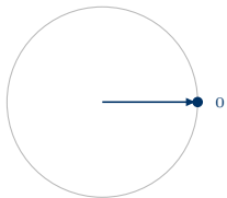
(a) \lambda_0 = 0
