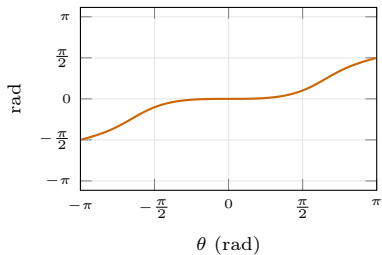
\angle F(e^{j\theta}) Circ. unit.
