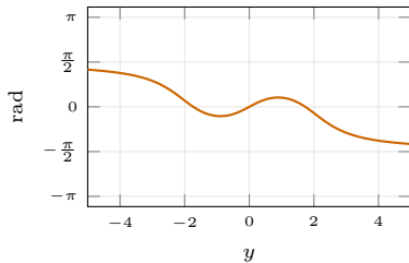
\angle F(e^{j\theta}) Circ. unit.
