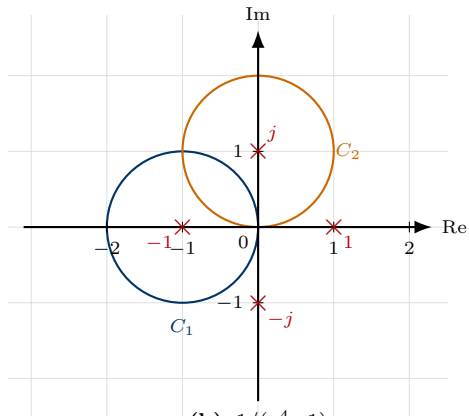
(b) 1/(z^4 - 1)
