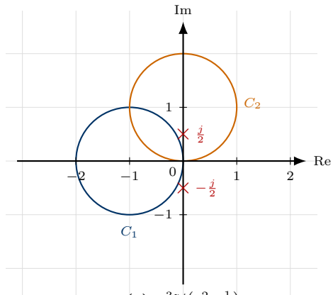
(a) e^{3z}/(z^2 + \frac{1}{4})
