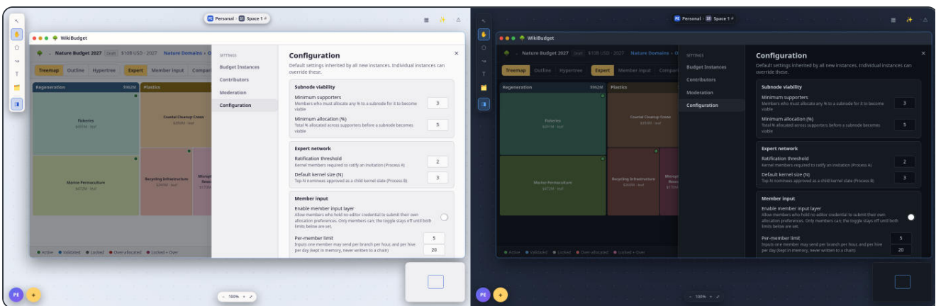
59. Settings, Configuration: a “Member input” toggle, a per-member limit and a pending cap. No proof-of-work control.
