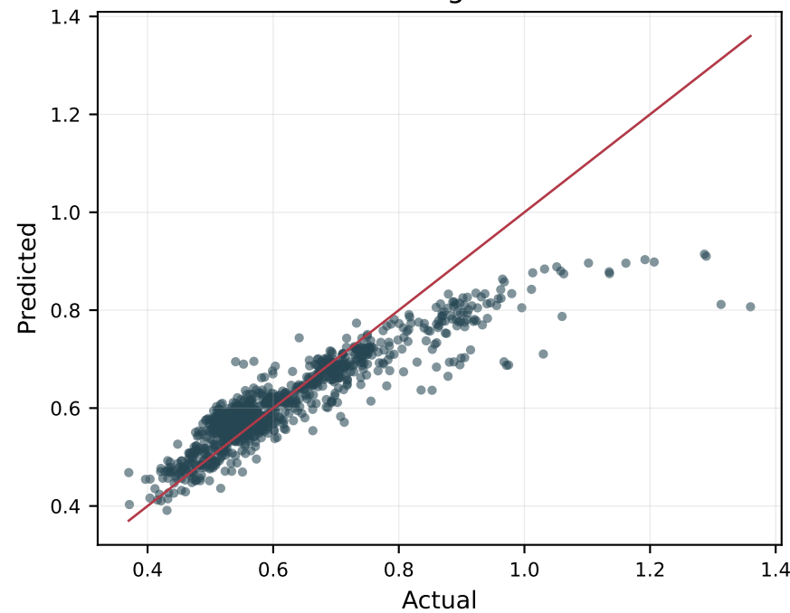
Extra Trees
