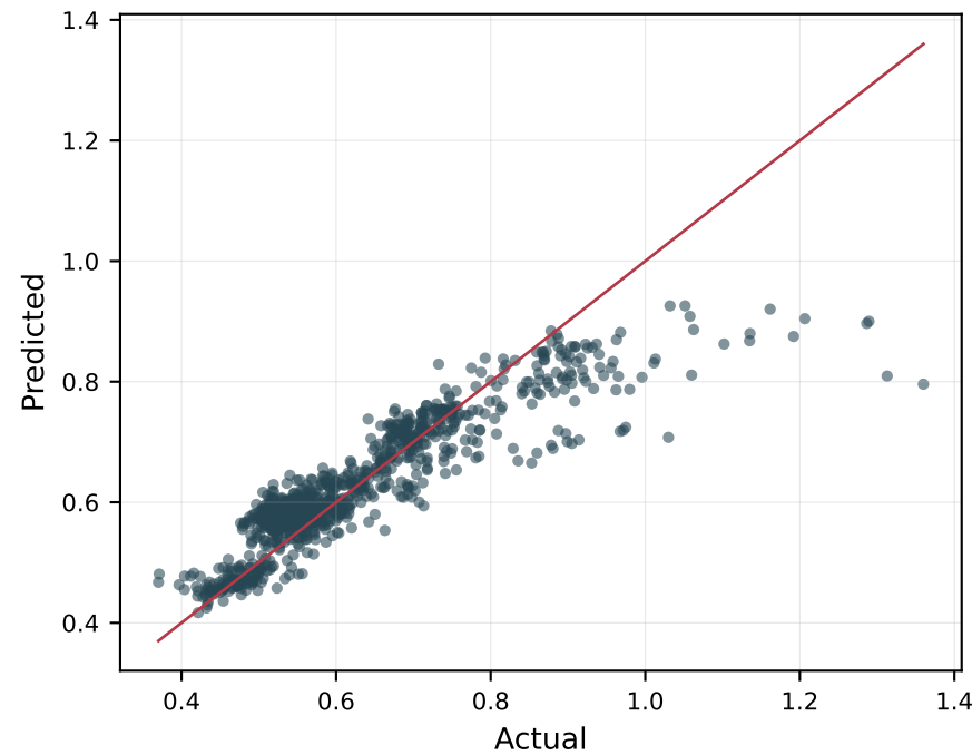
XGBoost
