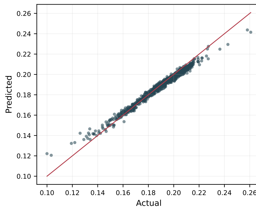
XGBoost
