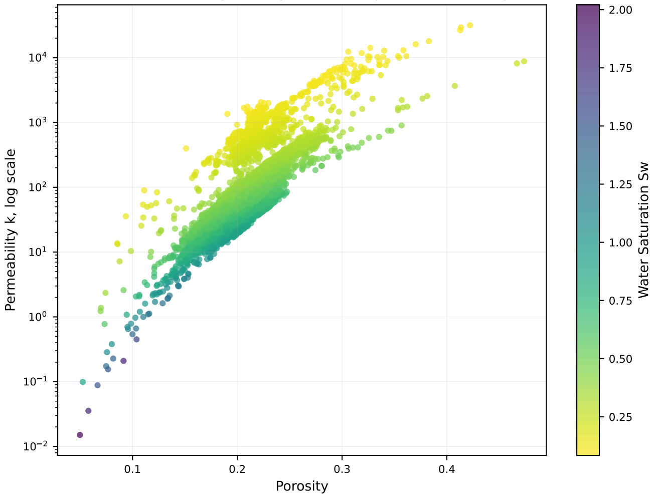
Reservoir Quality Crossplot: Porosity vs Permeability
