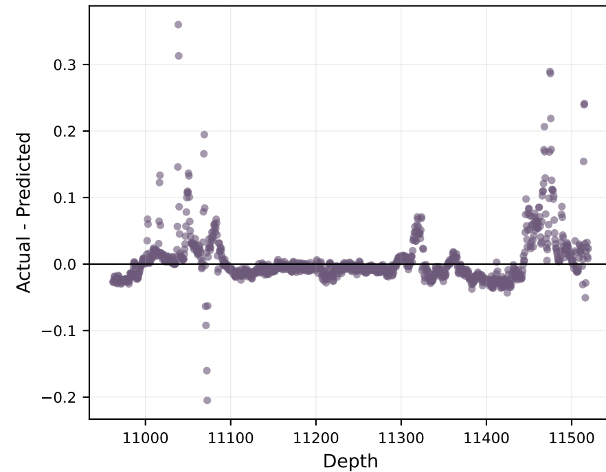
Water Saturation Sw Residual by depth
