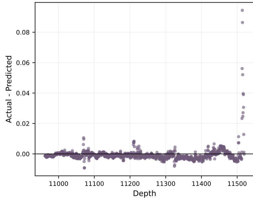
Porosity Residual by depth
