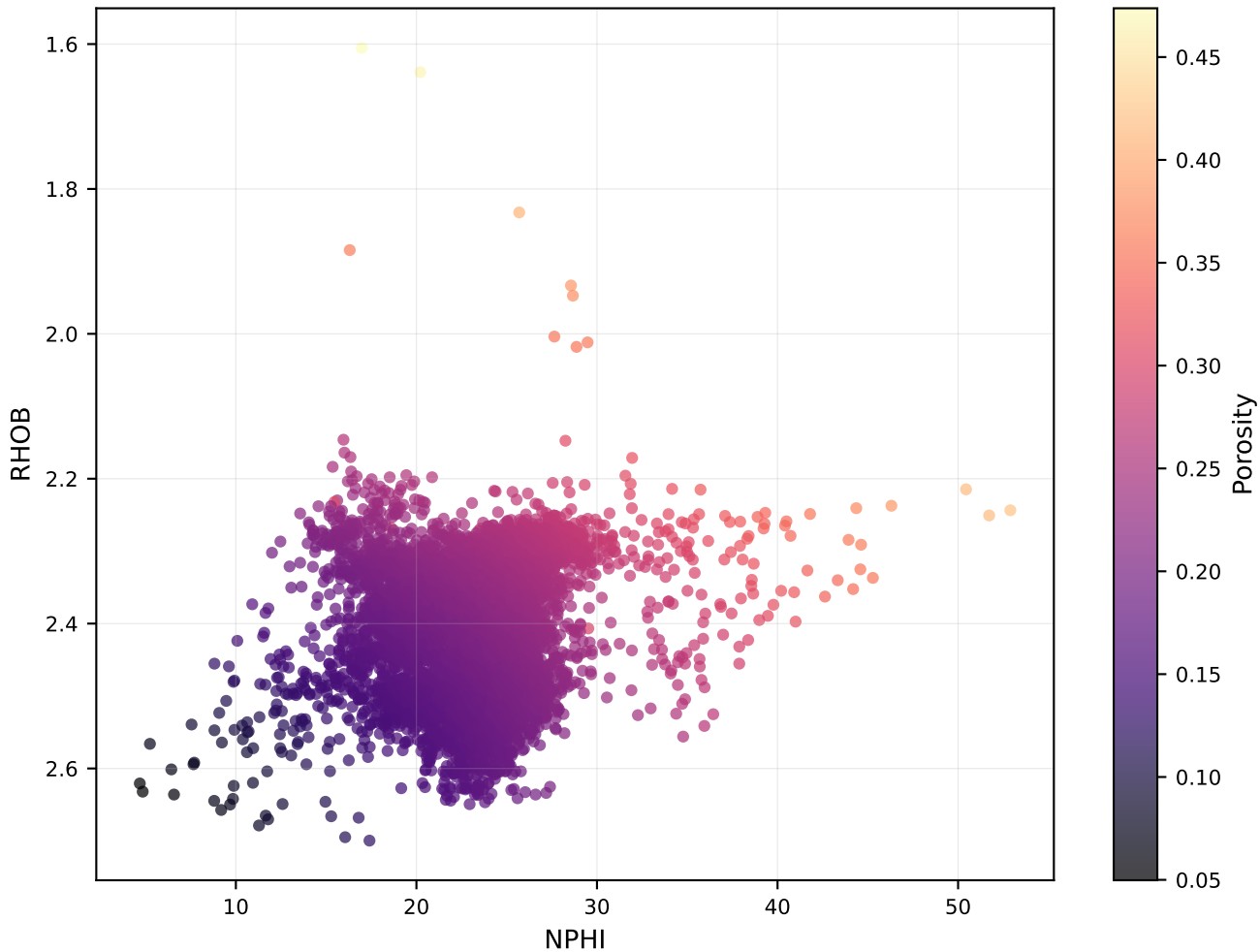
Neutron-Density Crossplot Colored by Porosity
