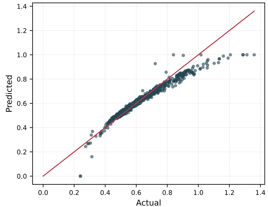
Water Saturation Sw Ridge Regression
